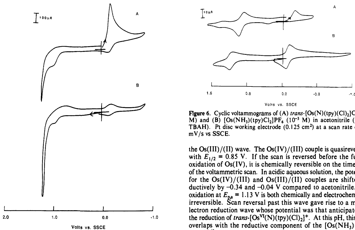
Figure 5. Cyclic voltammograms of (A) \text{trans-}[\text{Os}(\text{N})(\text{tpy})(\text{Cl})_2]\text{Cl} ( 10^{-2} \text{ M} ) and (B) [\text{Os}(\text{NH}_3)(\text{tpy})(\text{Cl})_2]\text{PF}_6 ( 10^{-2} \text{ M} ) in 3 \text{ M HCl} . Glassy carbon disc working electrode ( 0.07 \text{ cm}^2 ) at a scan rate of 200 \text{ mV/s} vs SSCE.
