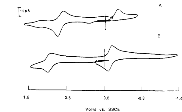
Figure 6. Cyclic voltammograms of (A) \text{trans-}[\text{Os}(\text{N})(\text{tpy})(\text{Cl})_2]\text{Cl} ( 10^{-3} \text{ M} ) and (B) [\text{Os}(\text{NH}_3)(\text{tpy})(\text{Cl})_2]\text{PF}_6 ( 10^{-3} \text{ M} ) in acetonitrile ( 0.1 \text{ M TBAH} ). Pt disc working electrode ( 0.125 \text{ cm}^2 ) at a scan rate of 200 \text{ mV/s} vs SSCE.
