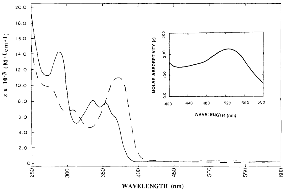
Figure 4. UV-vis spectra of [\text{Os}(\text{N})(\text{tpy})(\text{Cl})_2](\text{PF}_6) in \text{CH}_3\text{CN} solution (—) and in 0.1 \text{ M H}_2\text{SO}_4 (---).
